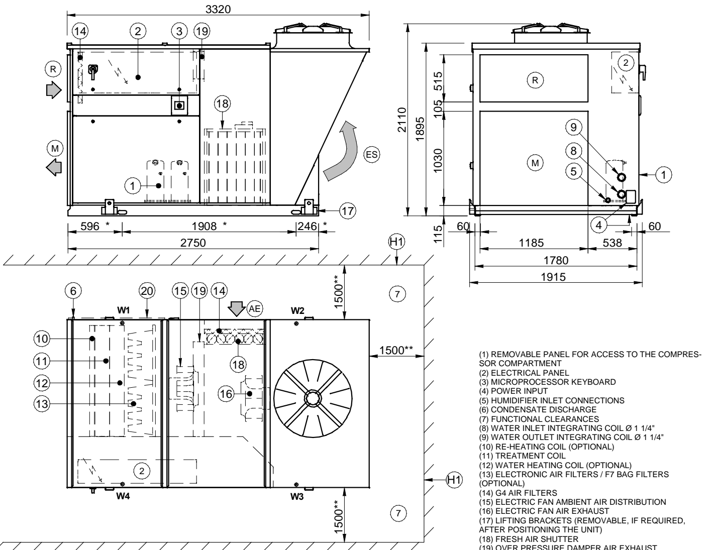
DIMENSIONAL DRAWING(1)
