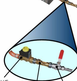
SOLENOID VALVE MEASURING DEVICE ADJUSTER MANUAL SHUT-OFF VALVE
