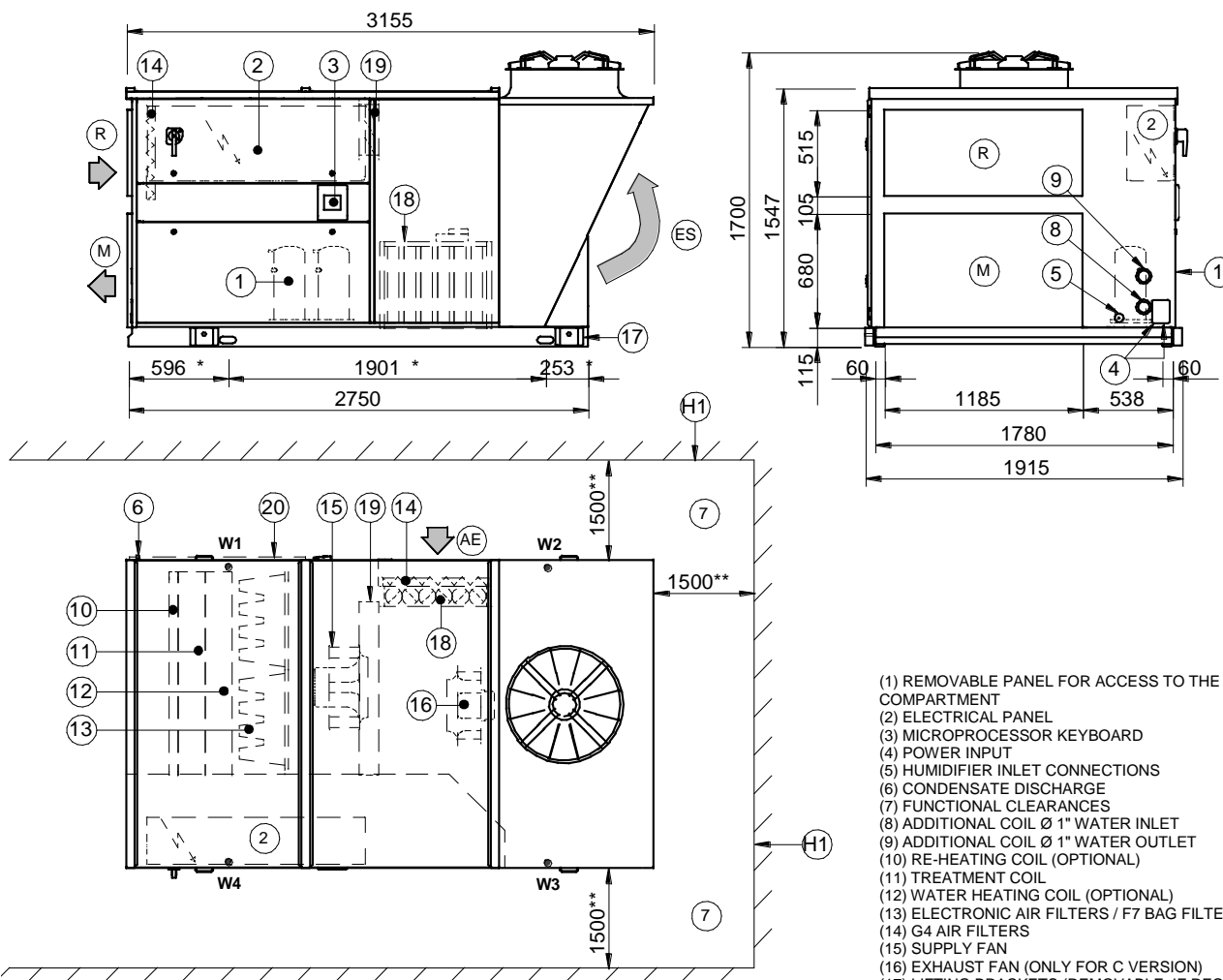
SIZE 82-102 DIMENSIONAL DRAWING(1)
