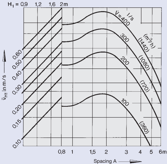
32 Diffuser arrangement: more than one row if B = 3.00 m
