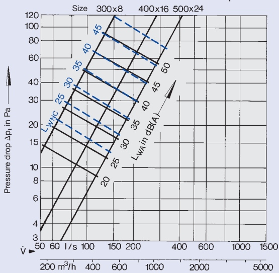
16 Sound Power Level and Pressure Drop VDW-...-H
