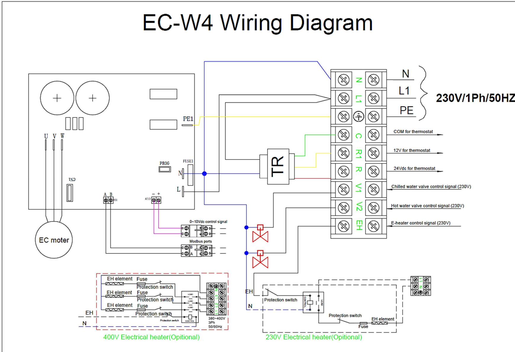
Wiring Diagram for PDWD-1000~1800-EC
